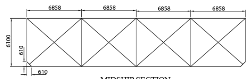
MIDSHIP SECTION
