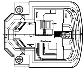
FORECASTLE DECK
